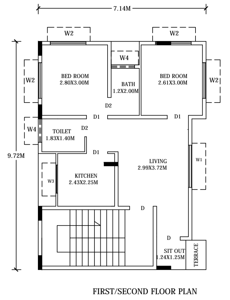
FIRST/SECOND FLOOR PLAN
